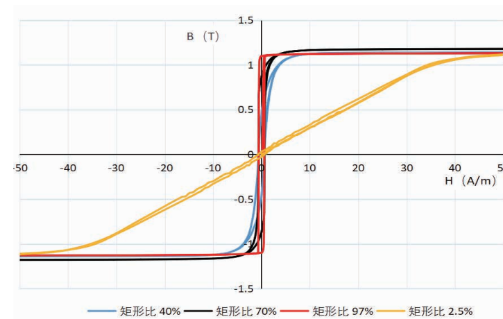
Hysteresis loop diagram of products with different squareness ratios
