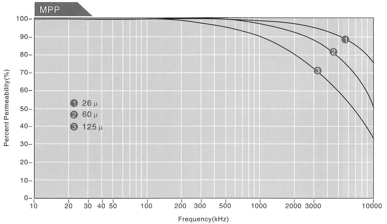
Permeability vs .Frequency
